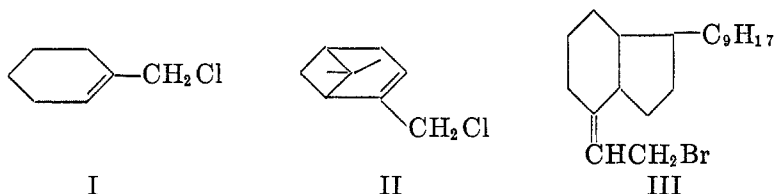
(e) Other reactions of allylic Grignard reagents
